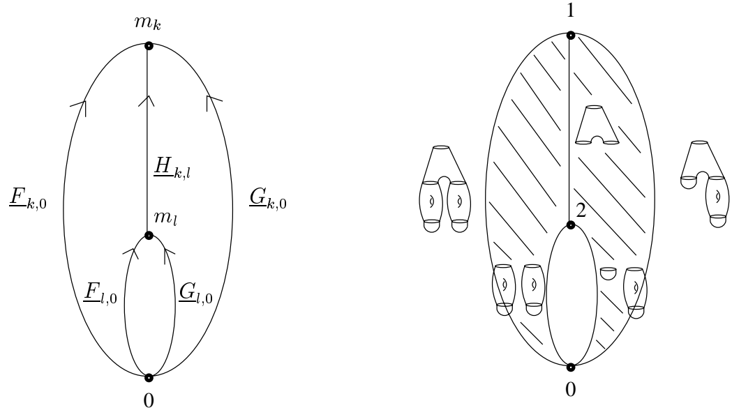
Figure 3.4: Homotopy H_{k,l}
