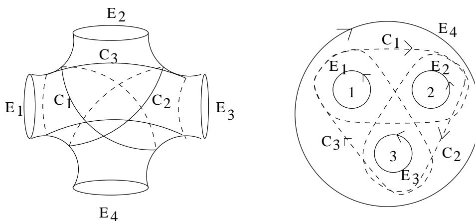
Figure 2.1: Lantern relation
