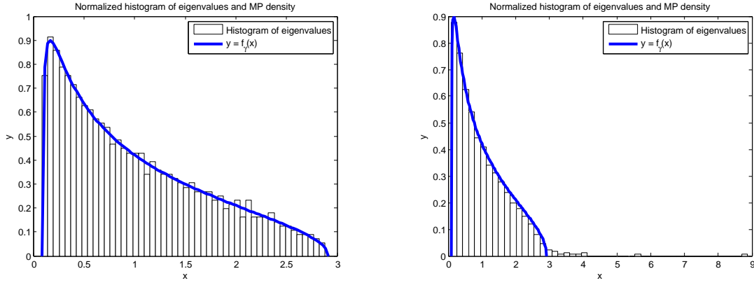
(a) Sample correlation: \mu_{(p)} = 0.088, \mu_{(1)} = 2.880 .
