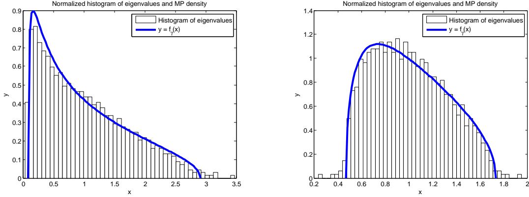
(a) X \stackrel{d}{=} Z^2 - \mathbb{E}Z^2 for Z \sim t_{1.5} , n = 2000 , p = 1000 , \gamma = 0.5 .
