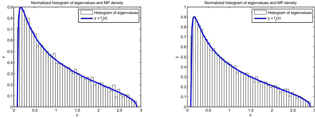
(a) Sample correlation: \mu_{(p)} = 0.086, \mu_{(1)} = 2.898 .
