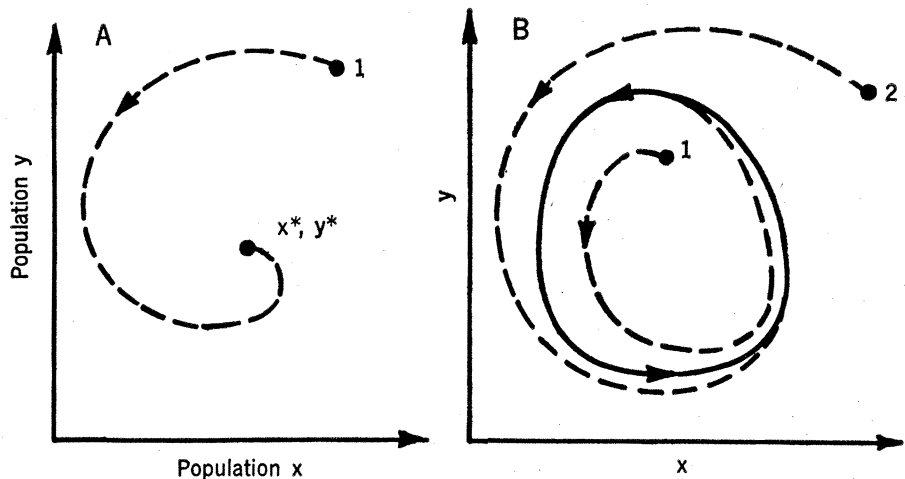
Fig. 1. Depiction of the "phase space" of two species, with populations x and y ; each point in the plane corresponds to some particular value of the two populations. In (A) the point x^*, y^* is a stable equilibrium point; if the populations are displaced from it (for example, to point 1), they tend in time to return, as exemplified by the dashed line. In (B) the solid curve is a stable limit cycle, and in equilibrium the two populations cycle around and around this trajectory, exhibiting well-defined and periodic oscillations in the population numbers; if displaced, either inside (for example, to point 1) or outside (for example, to point 2) their stable limit cycle, they tend to return to it, as illustrated by the dashed lines.
